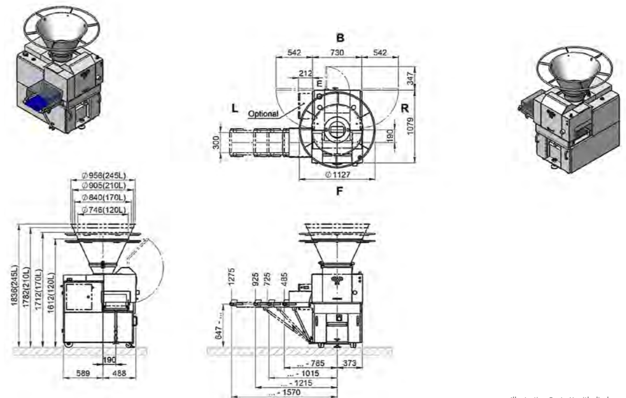
Illustration Parta U with discharge conveyor
