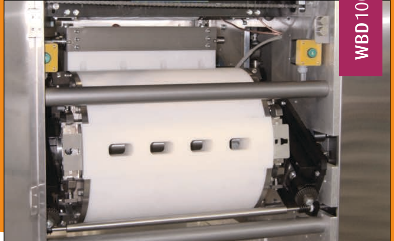
▣ Scaling Head
