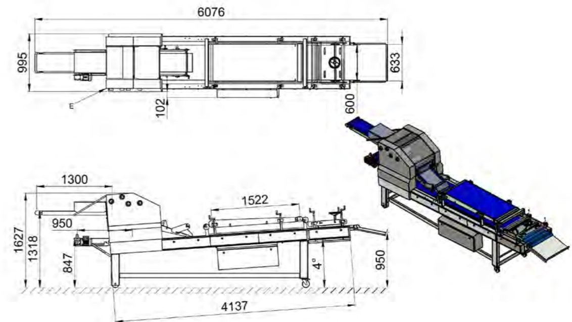
Illustration Combi UL inclined version with optional second pressure board and by pass
